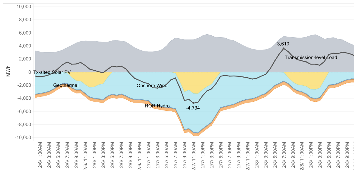
Figure 6 Transmission System: Net Load
