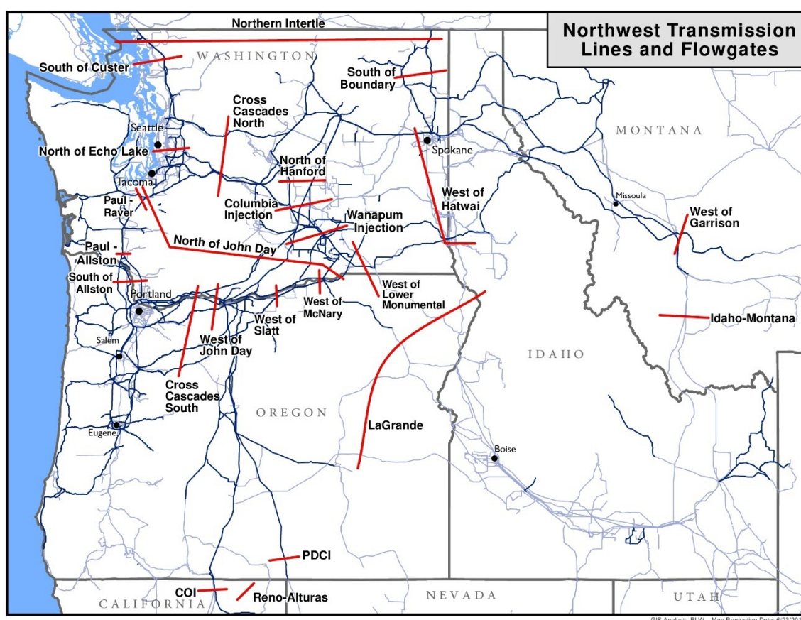
FIGURE 5-5: Pacific Northwest transmission system with BPA flowgates
