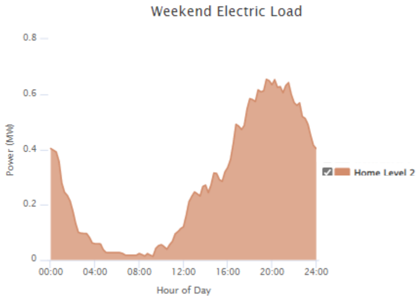
Figure 2.10 Estimated eastern Oregon weekend loading per 1,000 EVs
