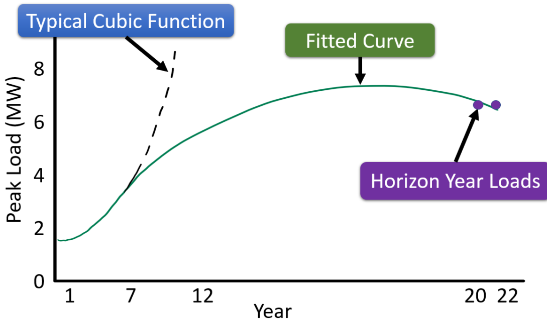
Figure 2.5 Cubic regression feeder S-curve fitted analysis
