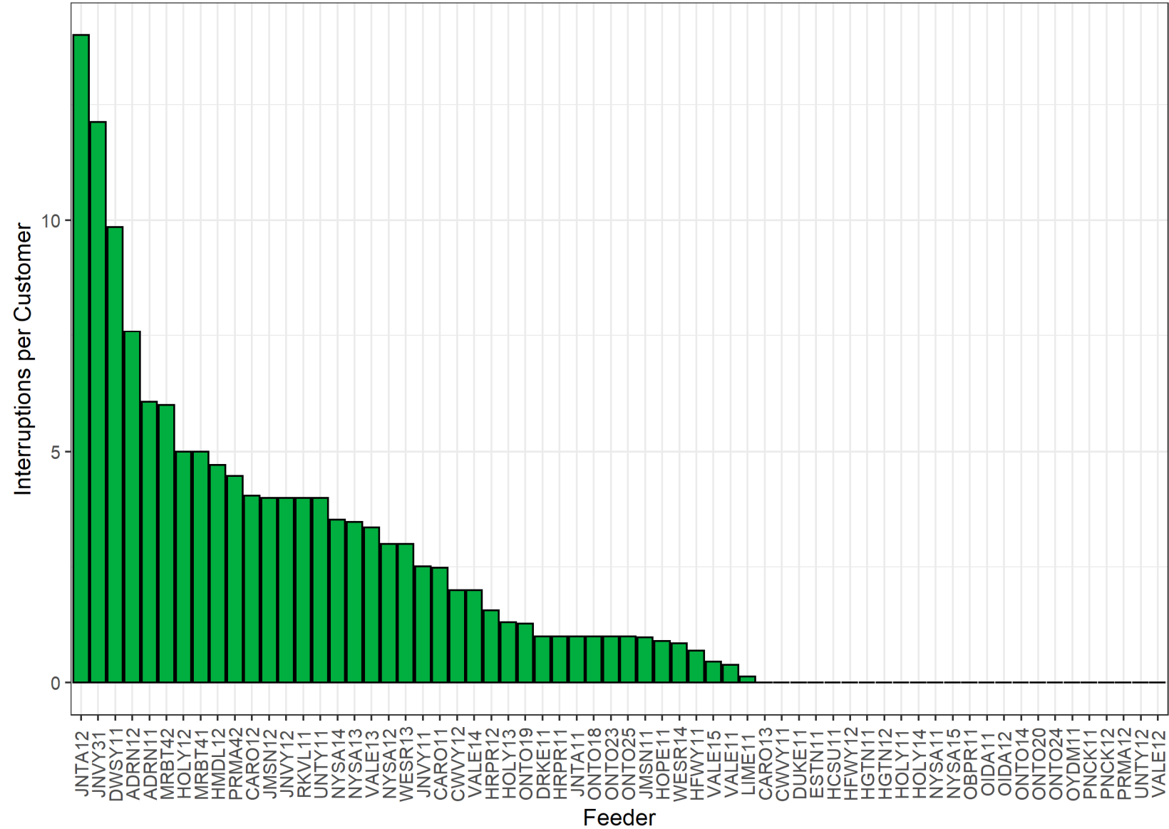
Figure 11 2021 Descending MAIFI by Circuit
