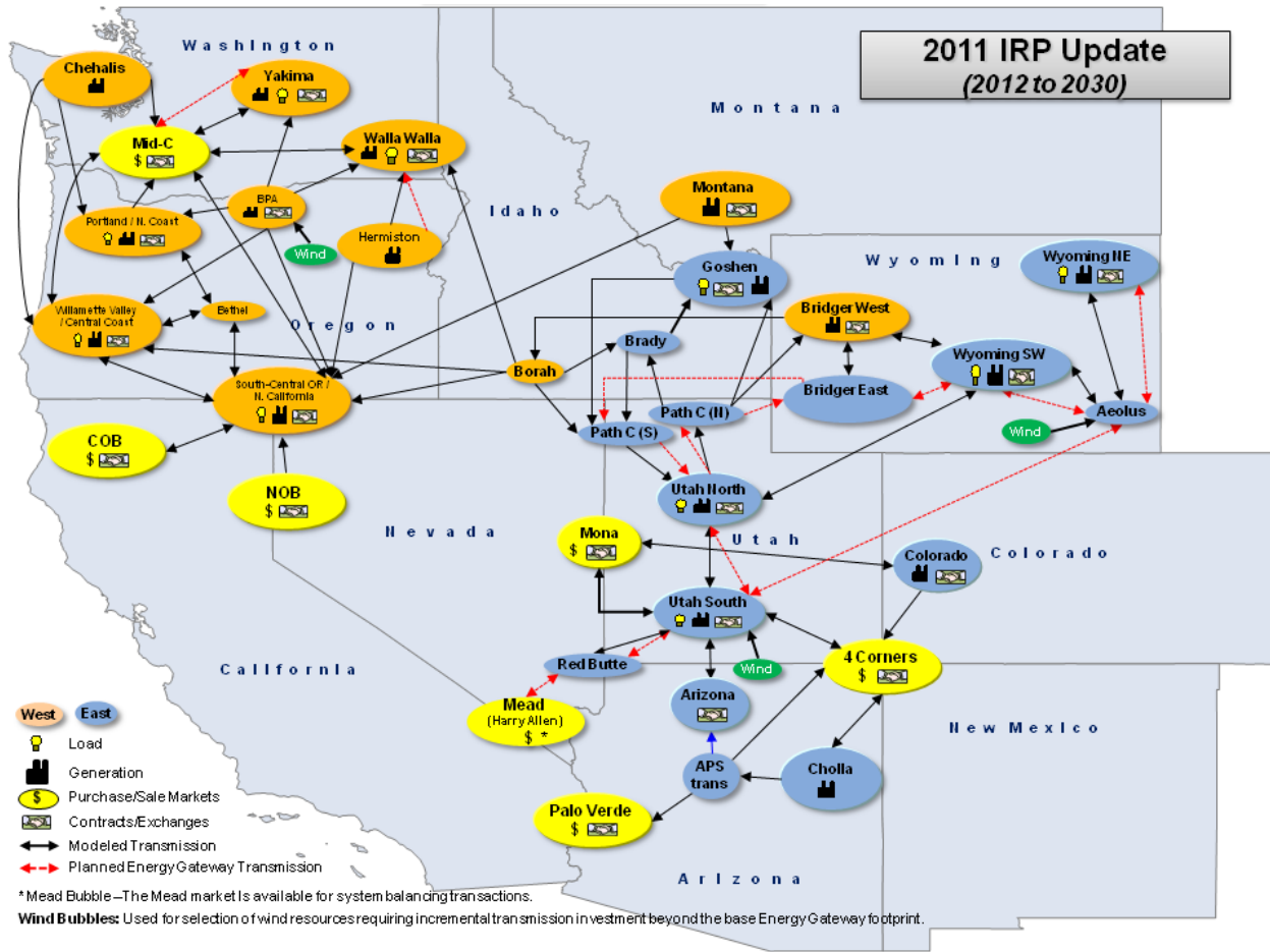
Figure 4.5 – Transmission Topology
