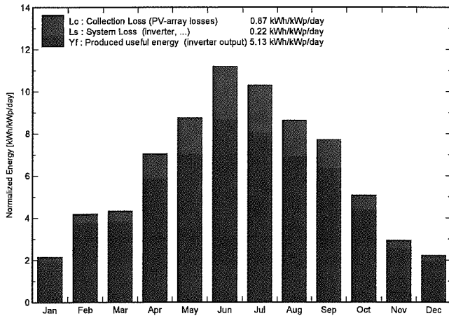
Normalized productions (per installed kWp): Nominal power 13097 kWp
